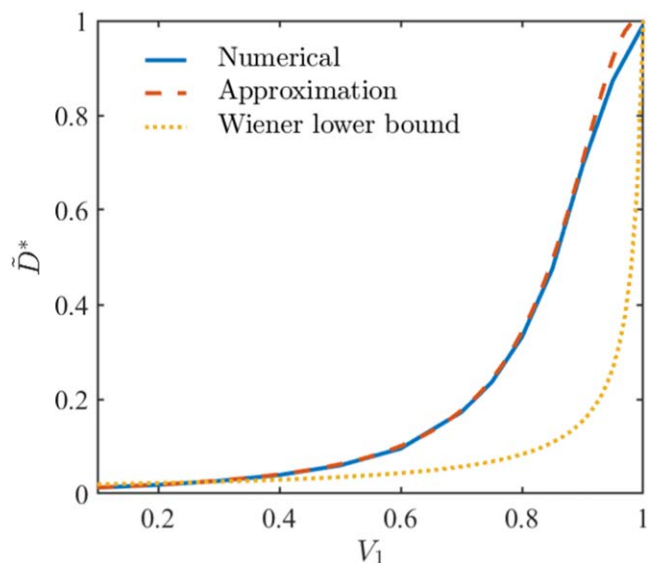
Figure 7. Steady-state effective diffusion coefficient \tilde{D}^* alternatively computed as the numerical solution of Eq. 29, the analytical expression 31 and the Wiener lower bound 53. It is plotted as function of the active material's volume fraction V_1 , for D_2/D_1 = 0.0178 .
